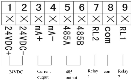
Wiring Diagram of Enhanced Integrated Type with Four-wire System
