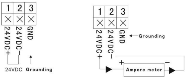
Wiring Diagram of Two-wire System Ampere Meter Diagram of Two-wire System
